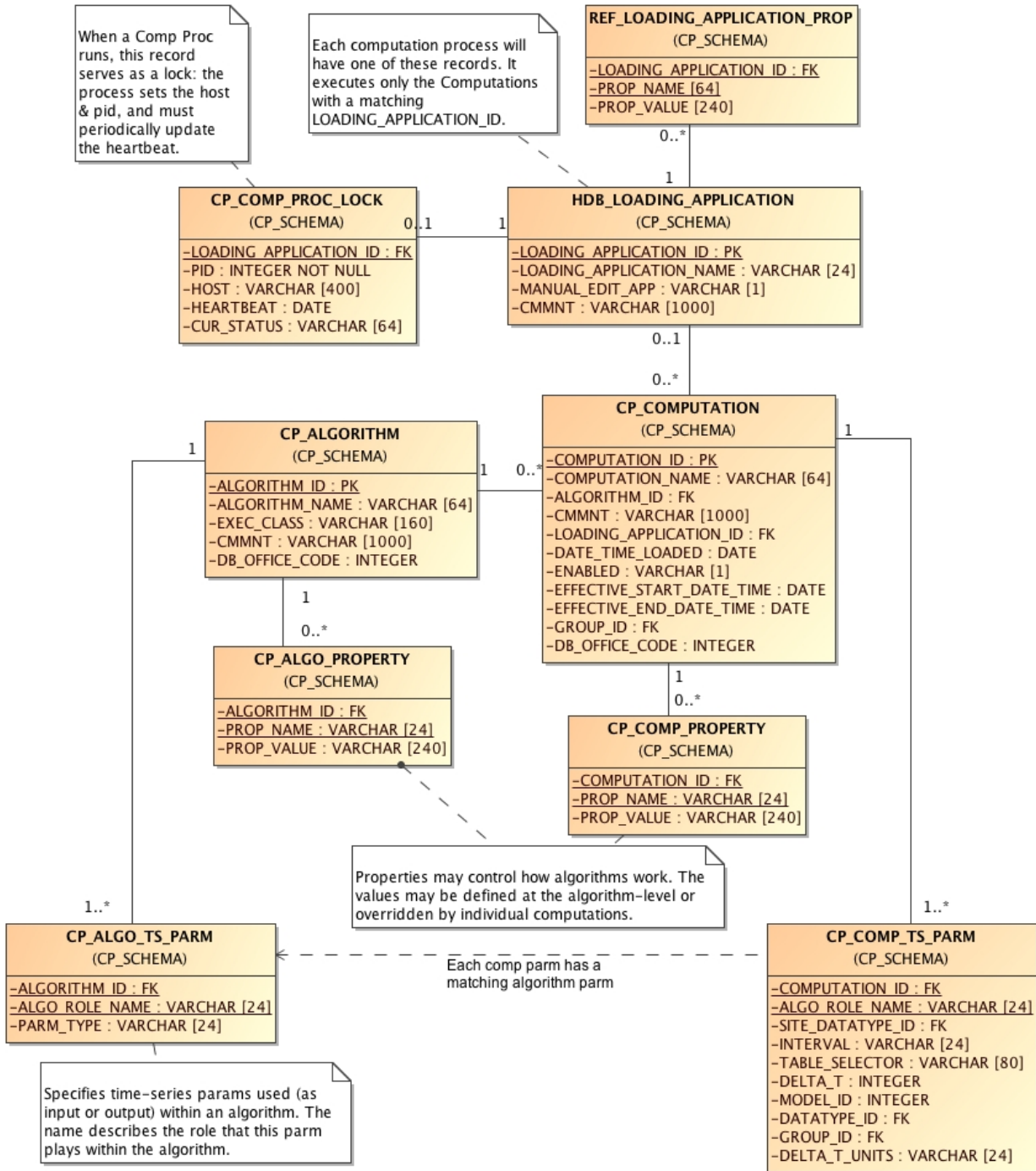
Figure 7: Computation Meta-Data Entity Relationship Diagram (ERD).
