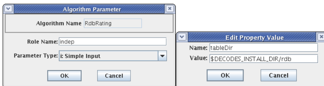
Figure 13: Algorithm Parameter and Property Dialogs.
