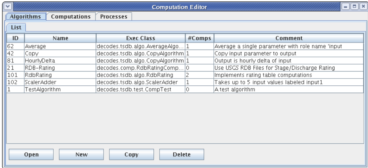
Figure 9: Computation Editor - Algorithms List Tab.
