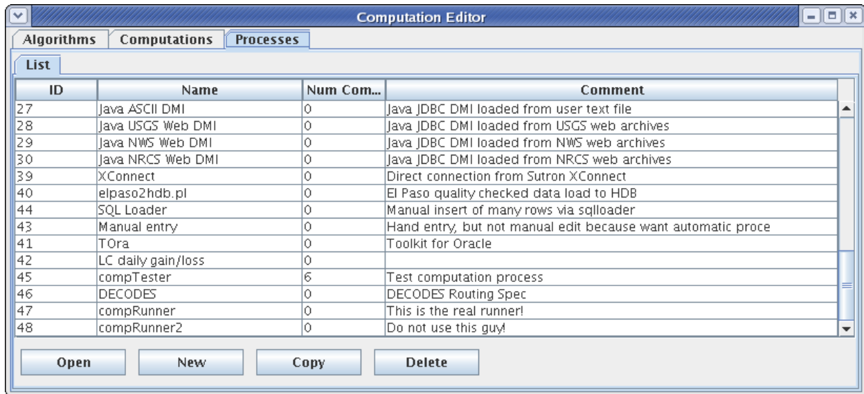
Figure 10: Computation Editor - Processes List Tab.
