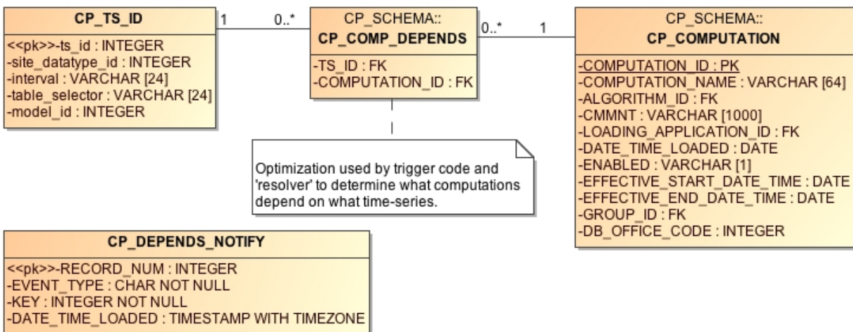
Figure 32: CP_COMP_DEPENDS table used to optimize relationship between time series and computations.
