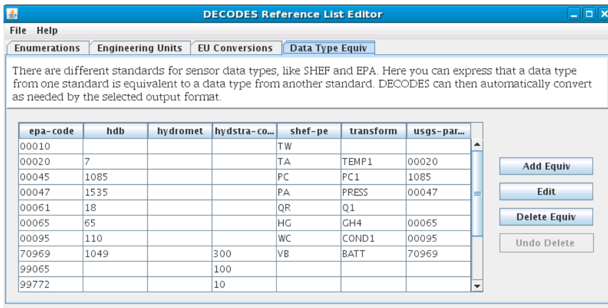
Figure 5: Reference List Editor - Data Type Equivalence Tab.
