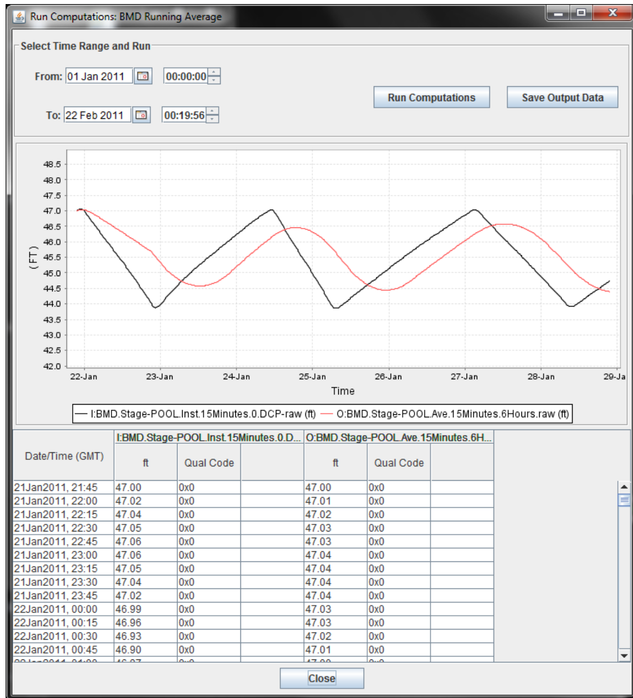
Figure 18: Run Computations Screen.
