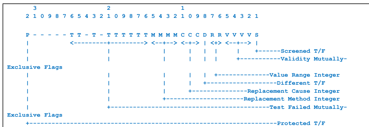
Figure 37: CWMS Time Series Value Quality Flags.
