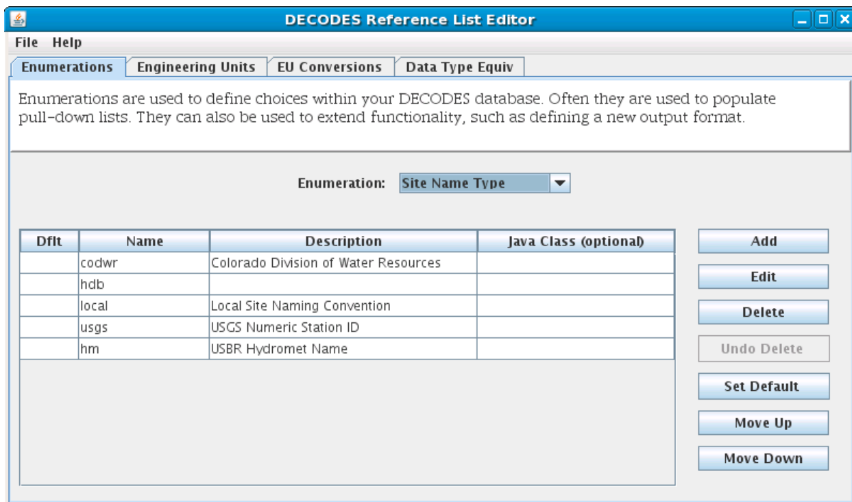
Figure 3: Reference List Editor being used to modify the Site Name Type Enumeration.
