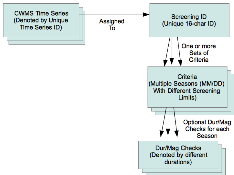
Figure 42: Logical Arrangement of CWMS Screening Records.
