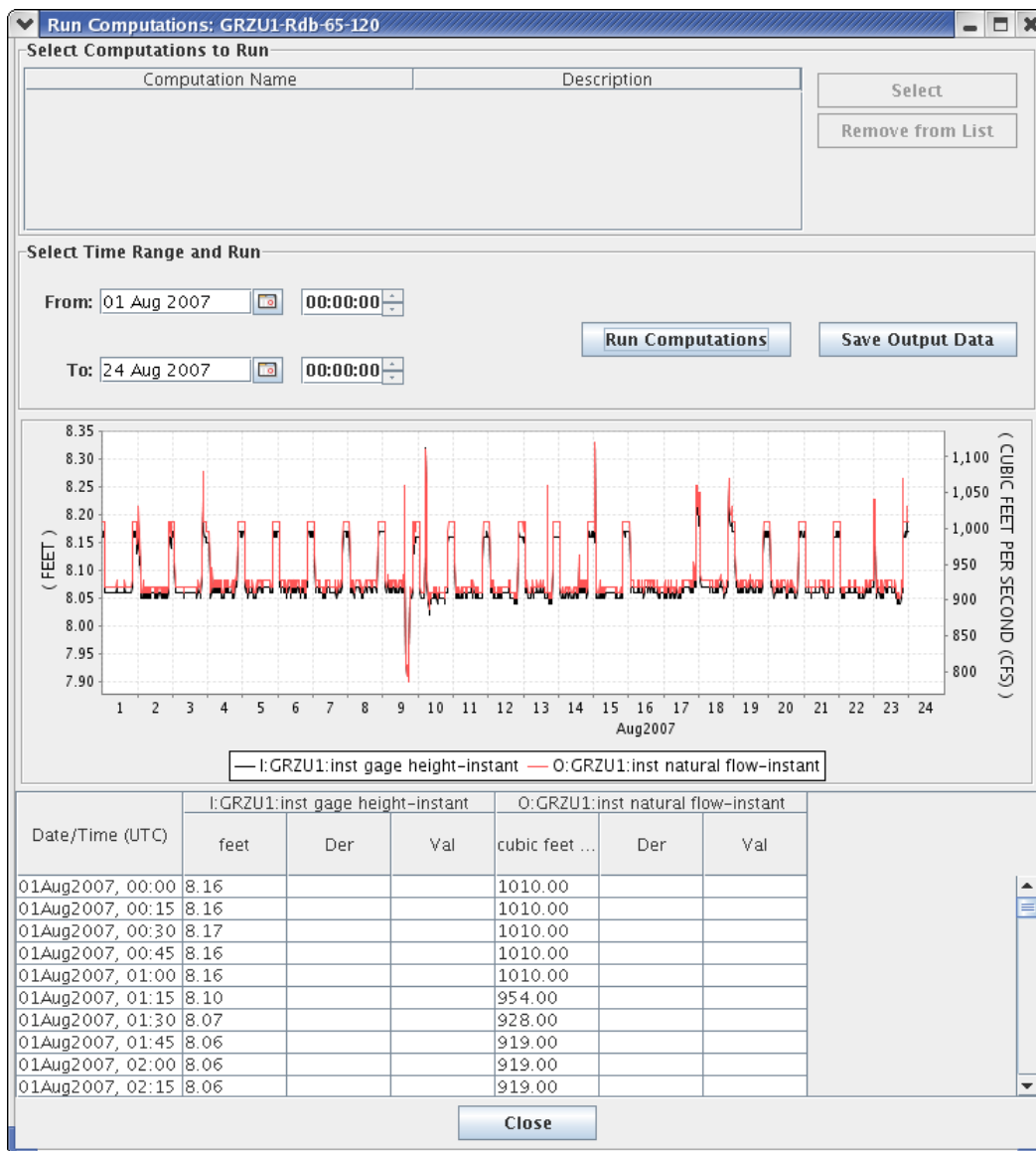
Figure 33: Interactive Run Computations GUI.
