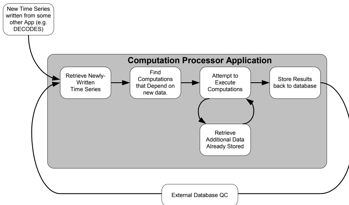
Figure 1: Workflow for the Computation Processor.
