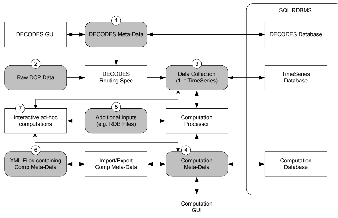
Figure 8: Workflow through the Provided Tools.
