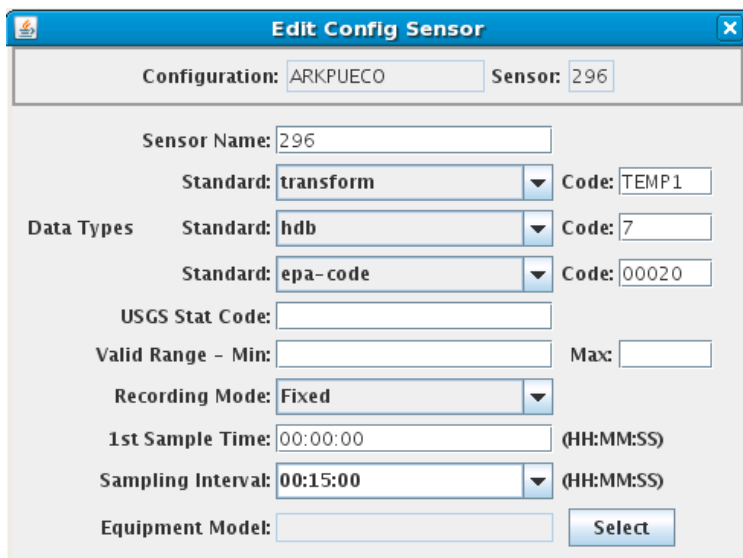
Figure 4: DECODES Edit Sensor Dialog, showing multiple data type codes.
