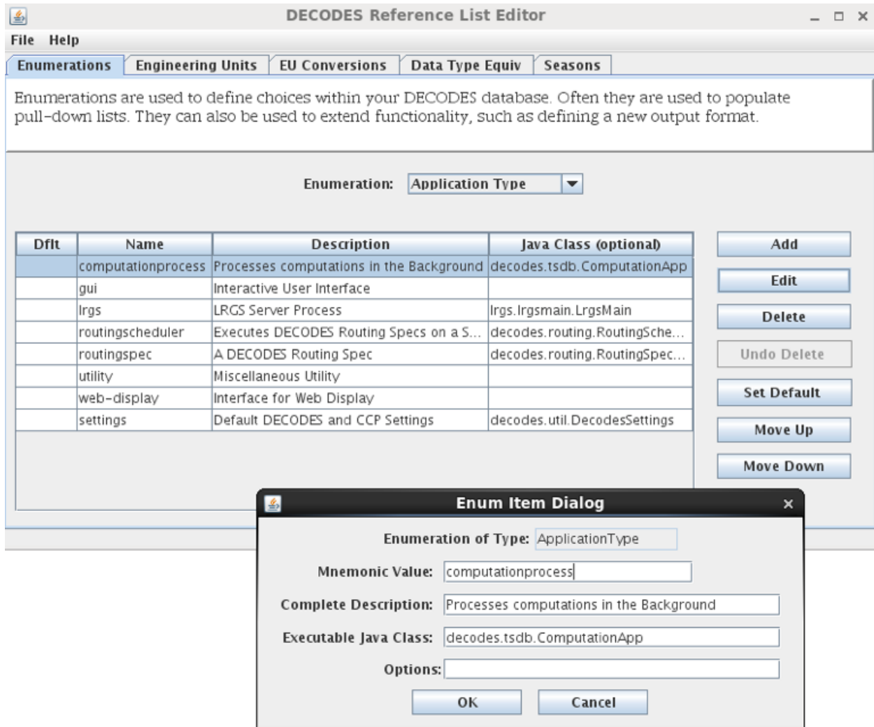
Figure 20: Application Type Enumeration
