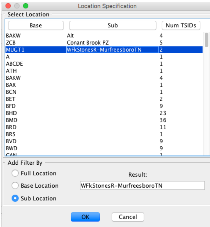
Figure 25: CWMS Group Editor Location Dialog.
