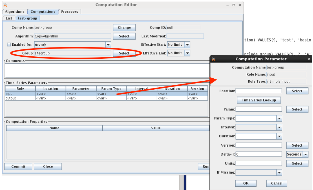
Figure 26: Using a Group in a Computation.
