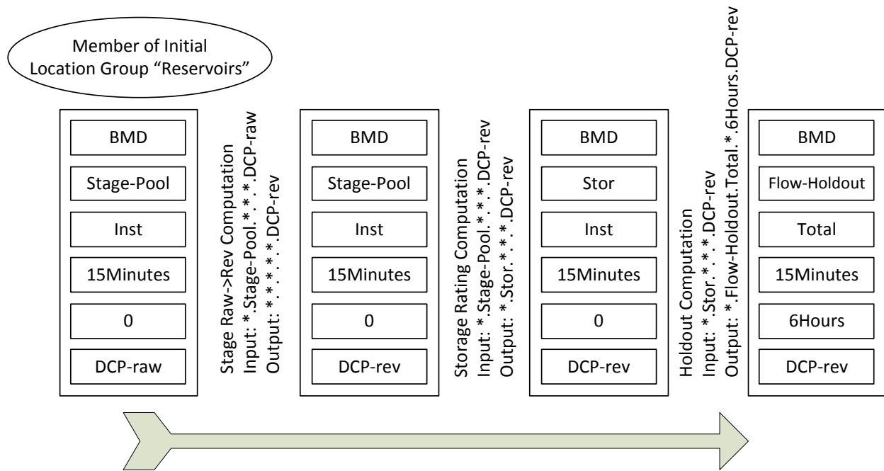
Figure 28: Chain of Computations with a Single Group.
