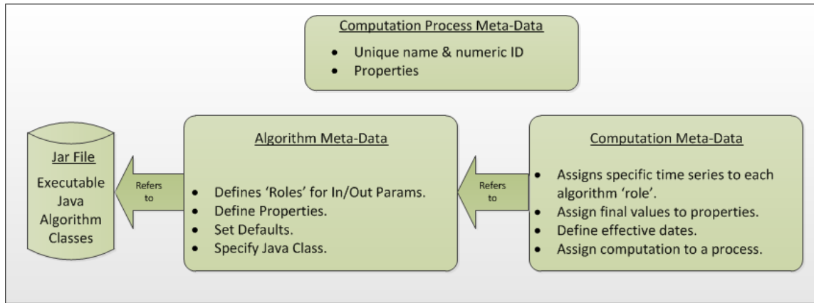
Figure 6: Logical Depiction of Computations Meta Data.
